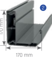
Extruded Frontal Gutter (Water-drain)
